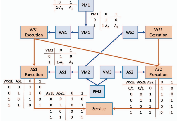
Fig. 3. The availability model of the example service in Bayesian network
