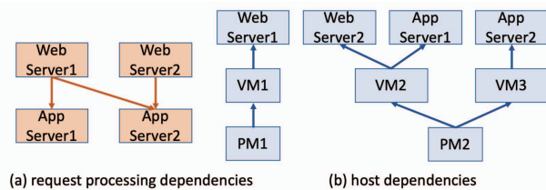
Fig. 1. The dependencies of the example service
