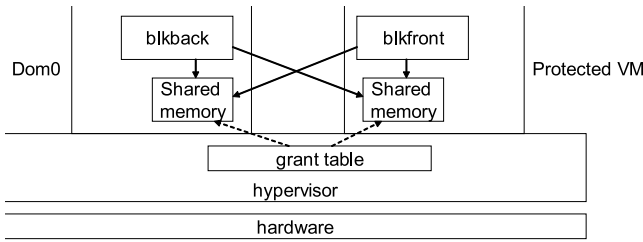
Fig. 10. Inter-domain shared memory for I/O operations in Xen.
