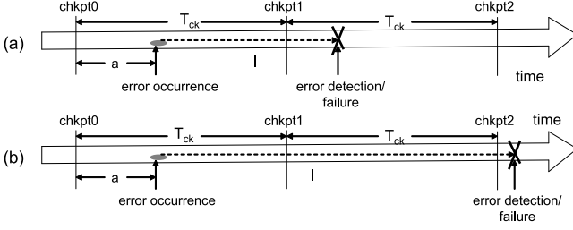
Fig. 4. Timeline of checkpoint corruption scenarios.
