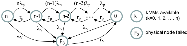
Fig. 6. The availability model for baseline ( n protected VMs).
