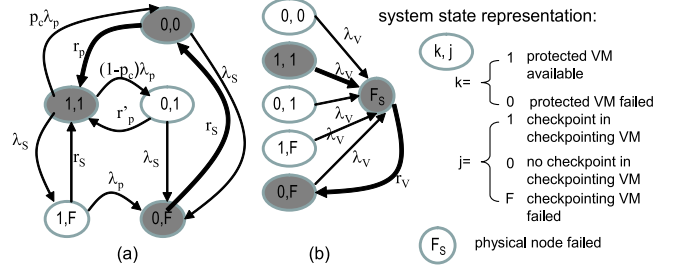
Fig. 5. Availability model for one protected VM (a) sub-model for transient failures of guest VMs, (b) sub-model for permanent failures and hypervisor failures.
