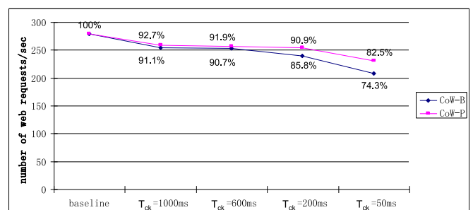
Fig. 9. Impacts of VM- \mu Checkpoint on Apache web server throughput (a percentage represents the ratio between the corresponding throughput and the baseline throughput, e.g., 82.5 percent=229.8/278.7).
