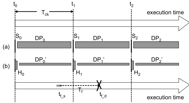
Fig. 2. Timelines for two checkpoint strategies: (a) COWB and (b) COWP.
