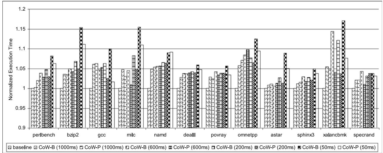
Fig. 8. Experiment results in terms of execution time of SPEC CINT 2006.
