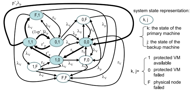
Fig. 7. The availability model for Remus (1 protected VM).
